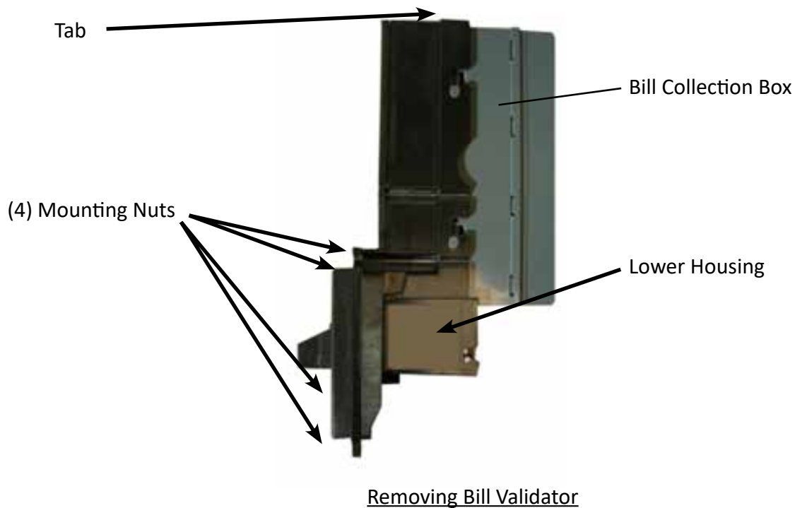
Figure 23 – Bill Validator
